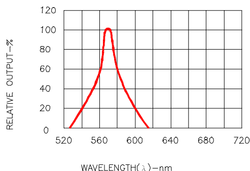
Fig.2 SPECTRAL RESPONSE
